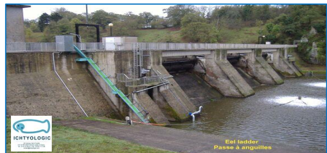
Dam of Apremont, Vie River \Delta h = 11.50 m
